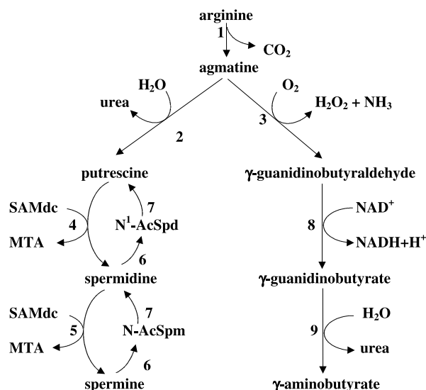
Fig. 1. Metabolism of agmatine. 1, arginine decarboxylase; 2, agmatinase; 3, diamine oxidase; 4, spermidine synthase; 5, spermine synthase; 6, spermidine/spermine acetyltransferase; 7, polyamine oxidase; 8, aldehyde dehydrogenase; 9, hydrolase; MTA, methylthioadenosine; \text{N}^1 -AcSpd, \text{N}^1 -acetylspermidine; N-AcSpm, N-acetylspermine; SAMdc, decarboxylated S-adenosyl- methionine
